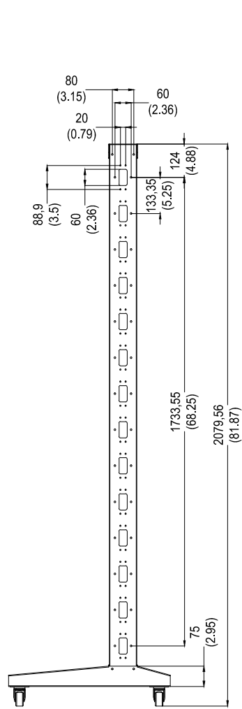
SIDE VIEW
