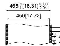
Mounting Distance
