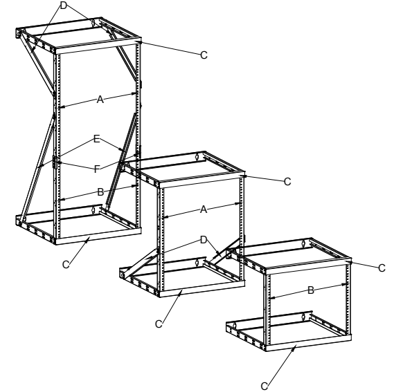
Assembly Diagram
