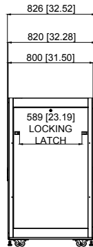
Right view
