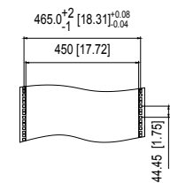
Mounting Distance
