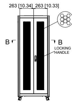
Rear view
