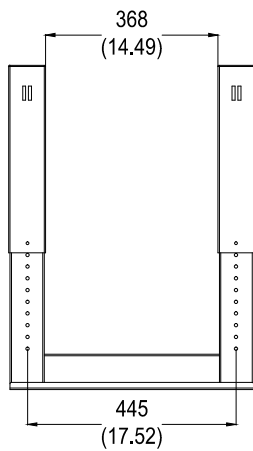
BOTTOM VIEW
